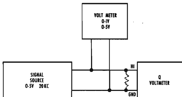
Figure VI-5 Q voltmeter calibration circuit
