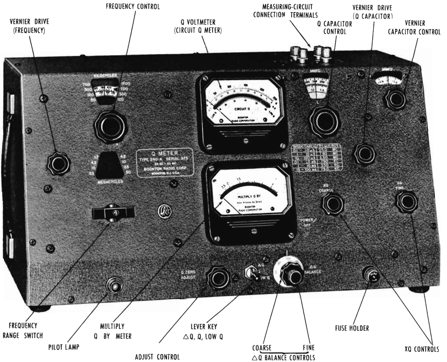
Figure I-1 Front view of Q Meter Type 260-A
